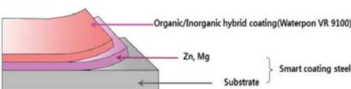
Protective coatings for Zn-Mg SMART Steel for Appliances
