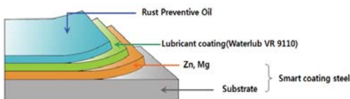
Lubricant coatings for Zn-Mg SMART Steel for Automotive
